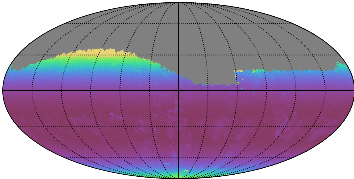
baseline_v2.1_10yrs Yr 1 g band: Min airmass
