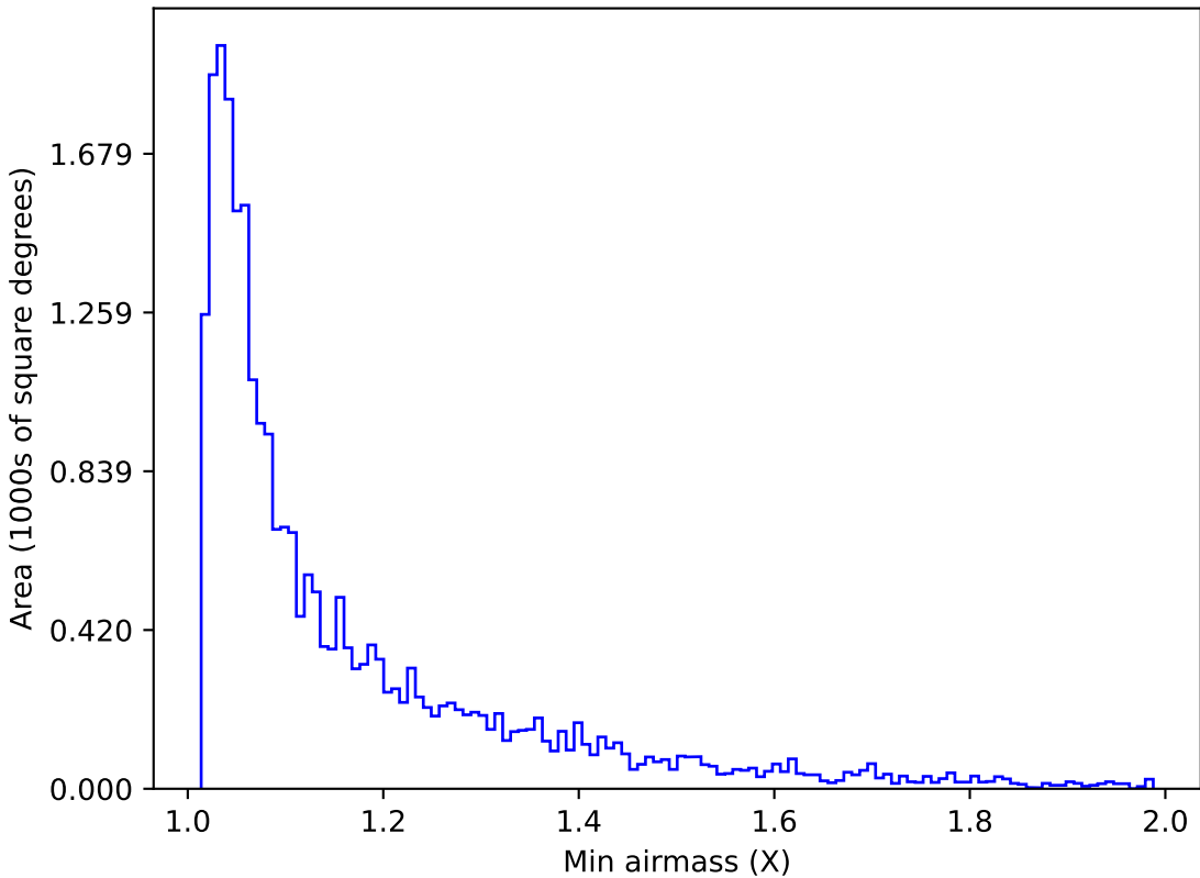
baseline_v2.1_10yrs Yr 1 g band: Min airmass
