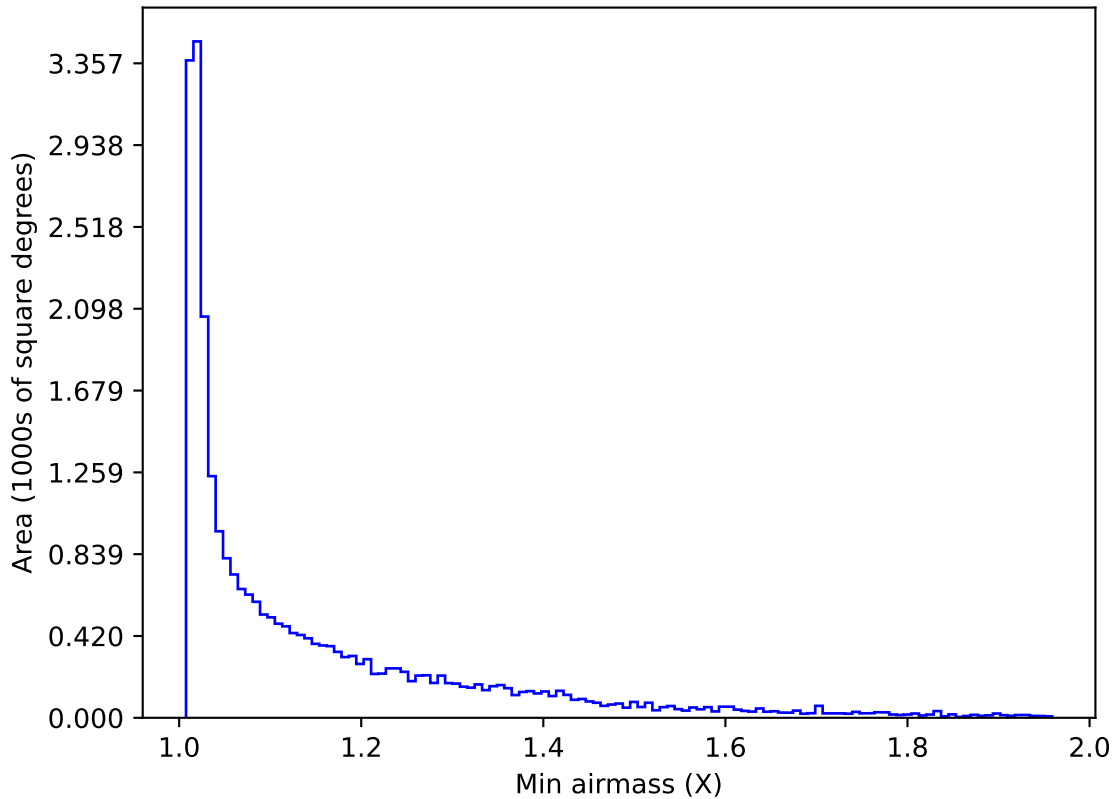
baseline_v2.1_10yrs Yr 1 all bands: Min airmass
