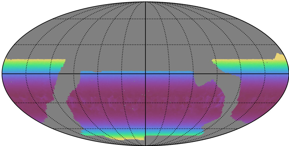
baseline_v2.1_10yrs WFD y band: Min airmass
