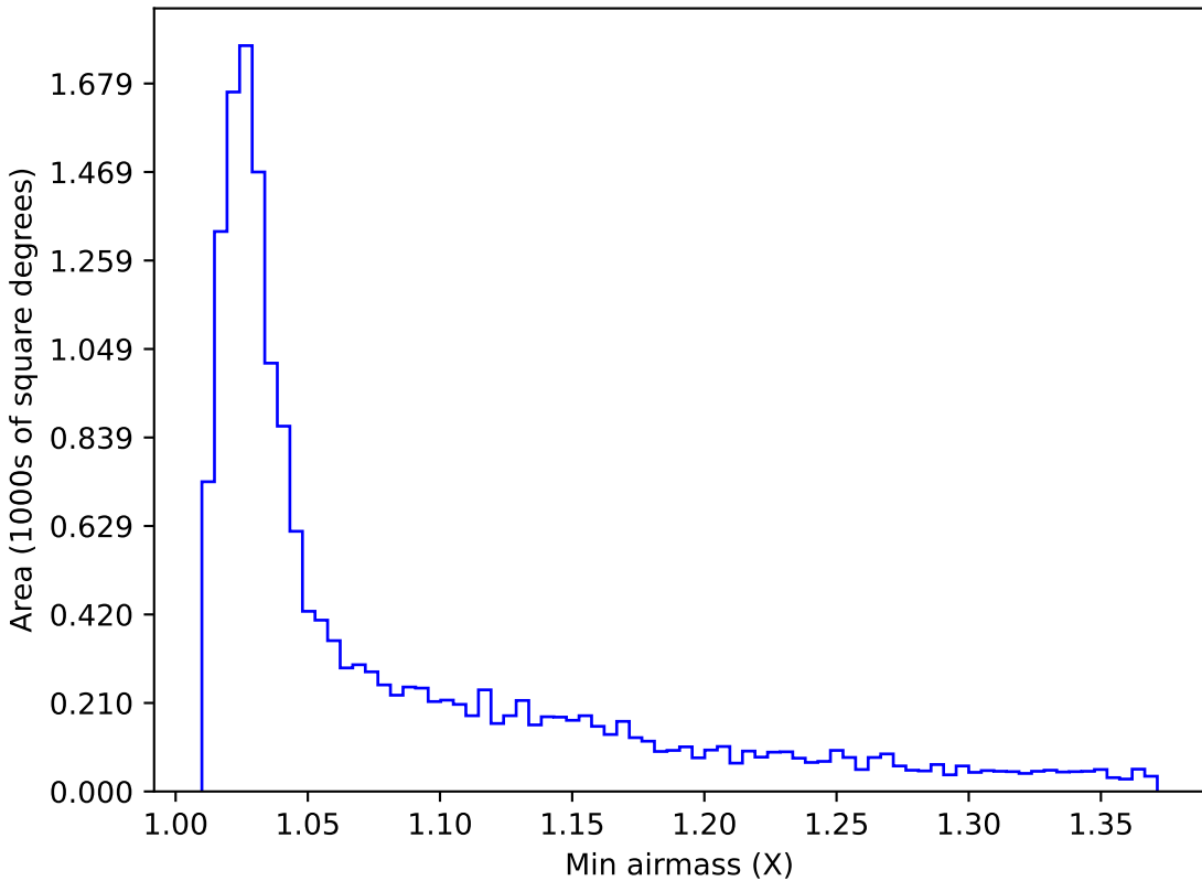
baseline_v2.1_10yrs WFD u band: Min airmass
