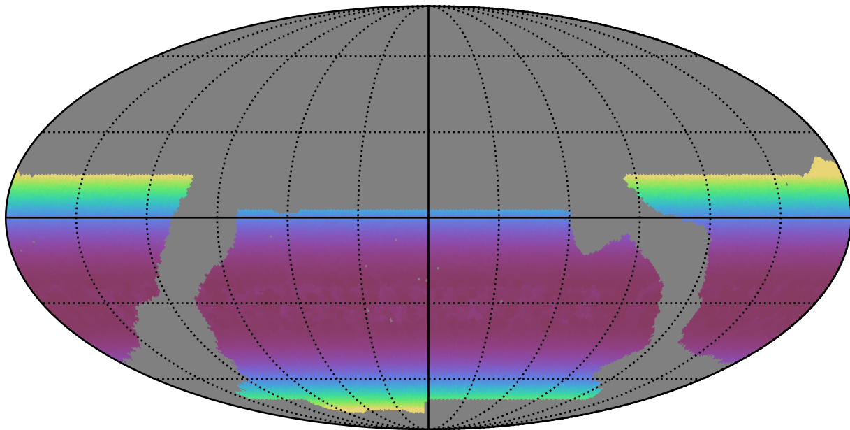
baseline_v2.1_10yrs WFD r band: Min airmass
