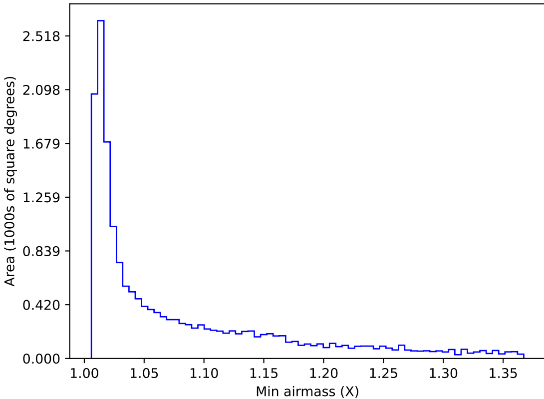
baseline_v2.1_10yrs WFD r band: Min airmass
