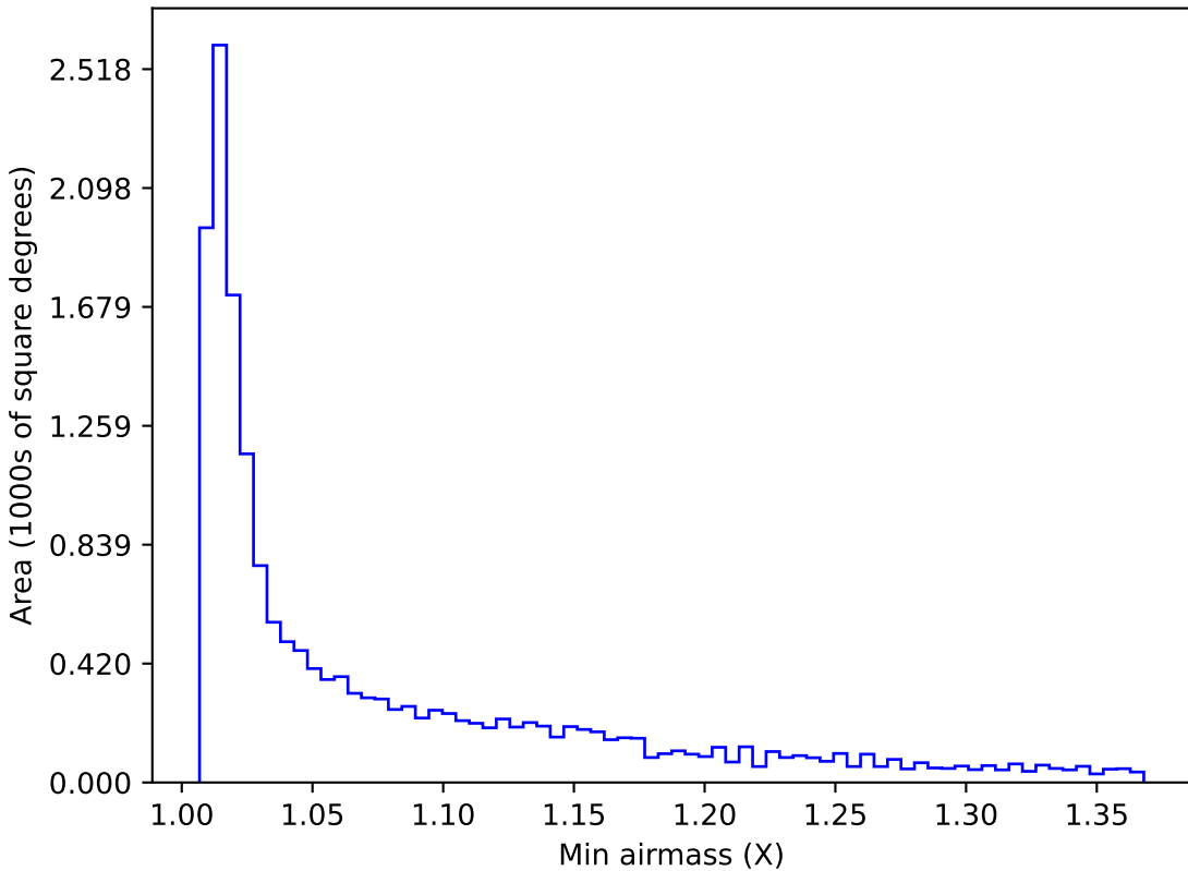
baseline_v2.1_10yrs WFD i band: Min airmass
