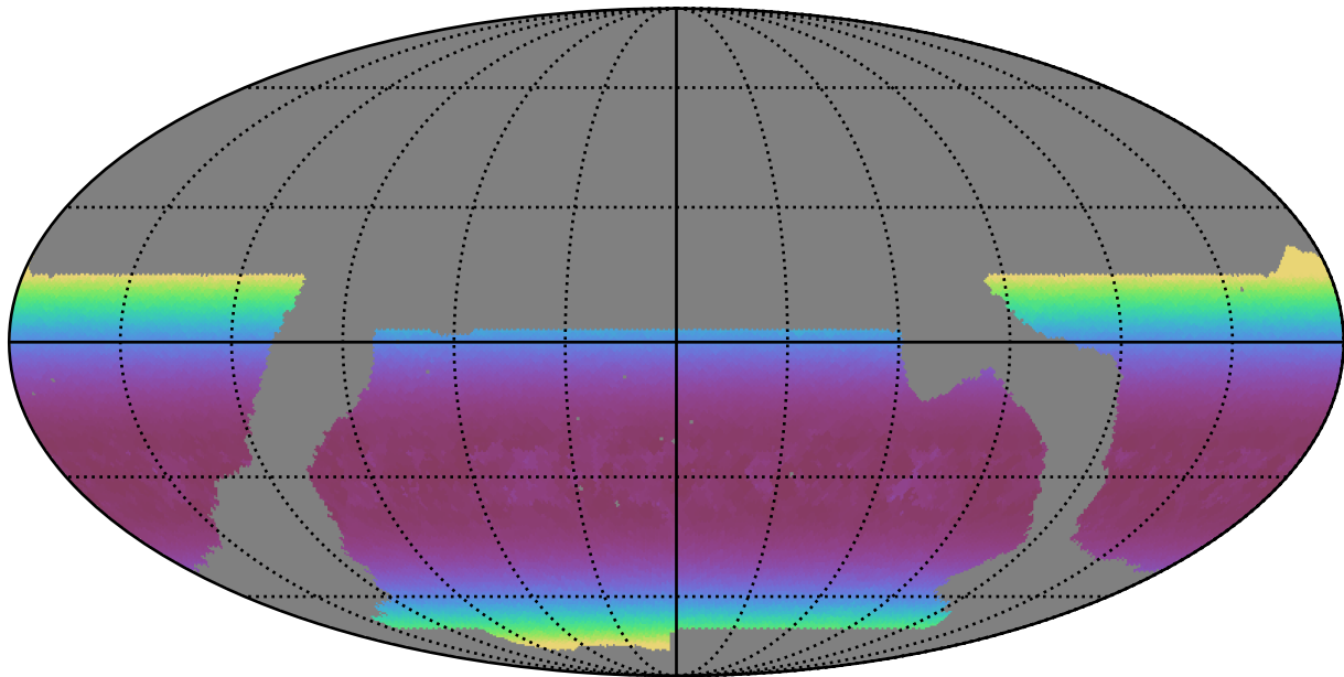
baseline_v2.1_10yrs WFD g band: Min airmass
