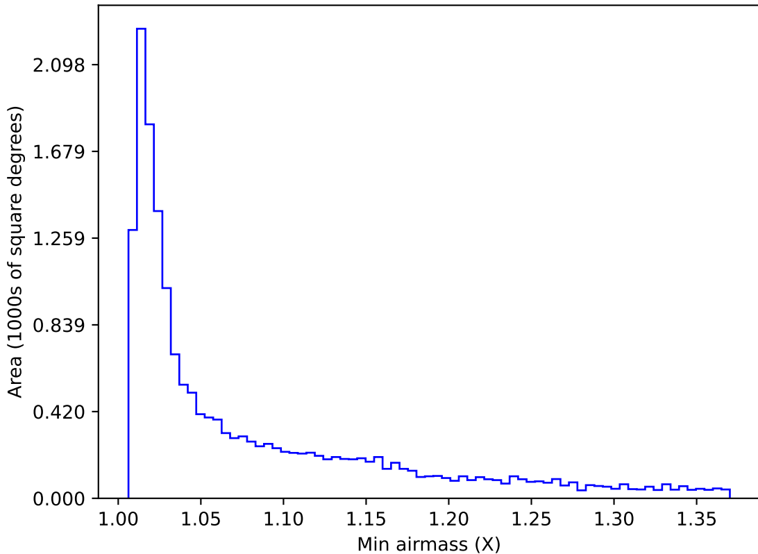
baseline_v2.1_10yrs WFD g band: Min airmass
