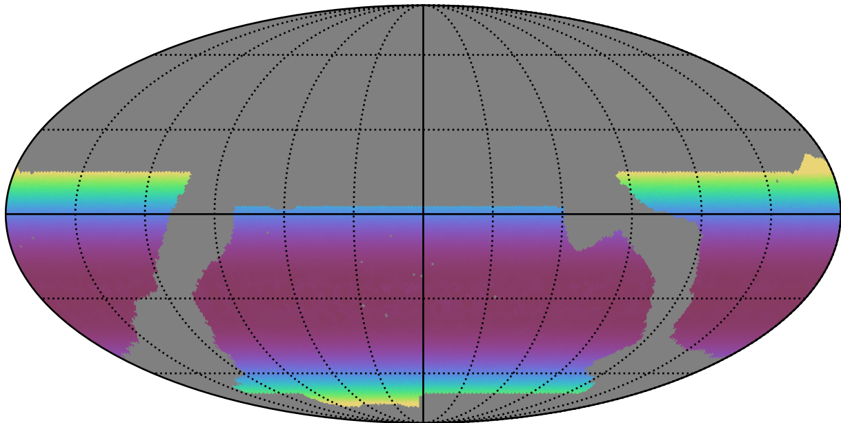
baseline_v2.1_10yrs WFD all bands: Min airmass
