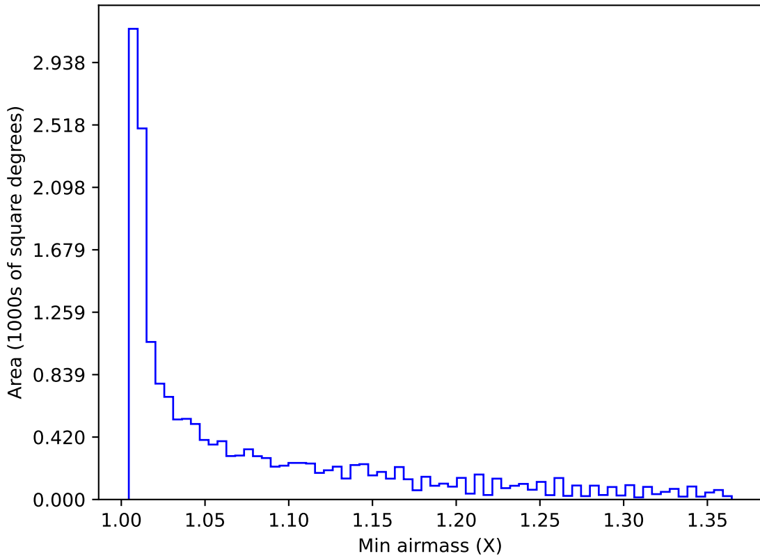
baseline_v2.1_10yrs WFD all bands: Min airmass
