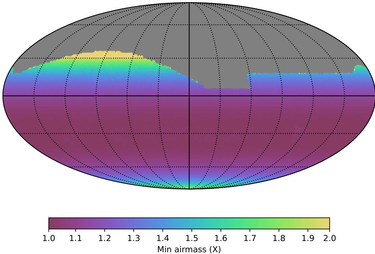
baseline_v2.1_10yrs All sky z band: Min airmass
