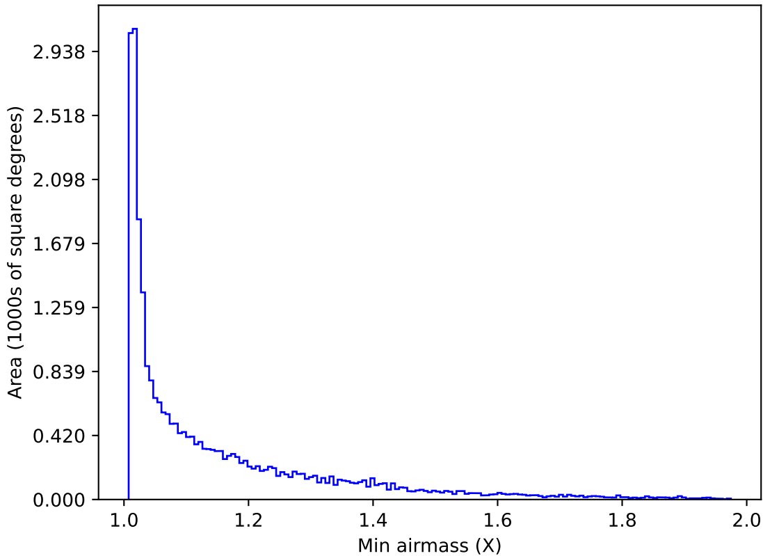
baseline_v2.1_10yrs All sky z band: Min airmass
