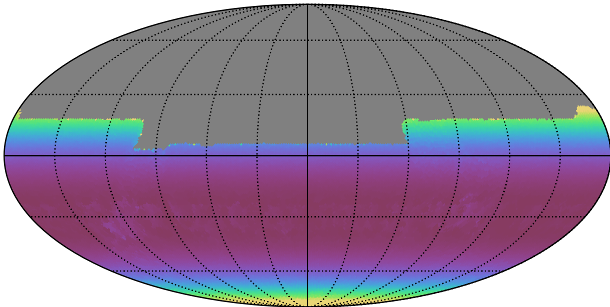
baseline_v2.1_10yrs All sky y band: Min airmass
