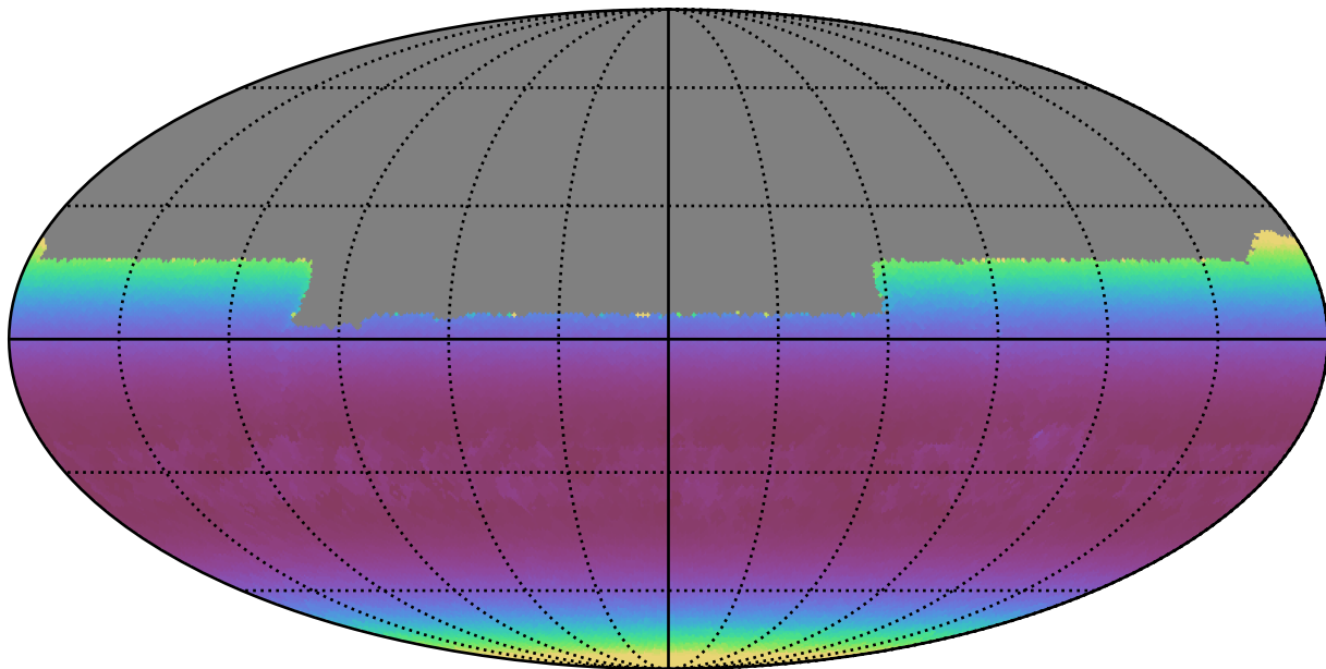
baseline_v2.1_10yrs All sky u band: Min airmass
