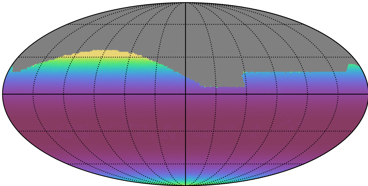
baseline_v2.1_10yrs All sky r band: Min airmass
