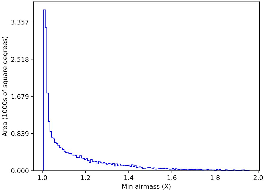
baseline_v2.1_10yrs All sky r band: Min airmass
