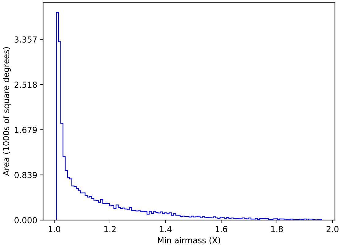
baseline_v2.1_10yrs All sky i band: Min airmass
