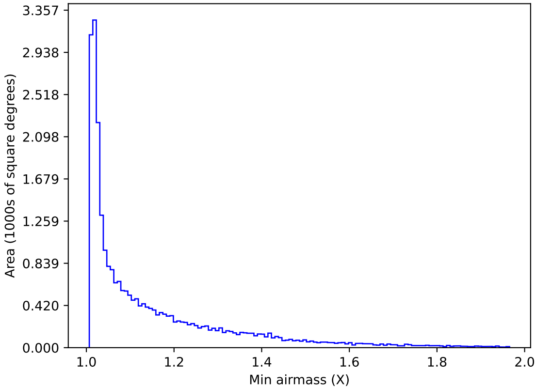
baseline_v2.1_10yrs All sky g band: Min airmass
