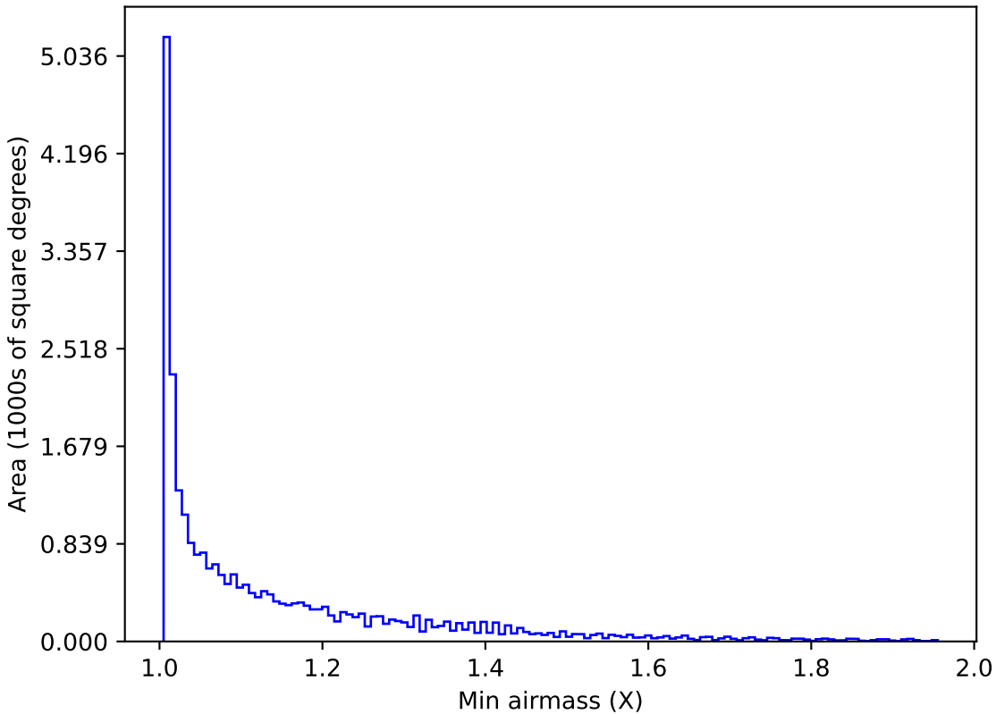
baseline_v2.1_10yrs All sky all bands: Min airmass
