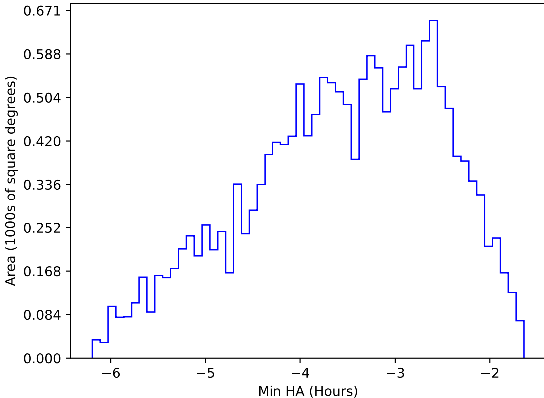
baseline_v2.1_10yrs WFD z band: Min HA
