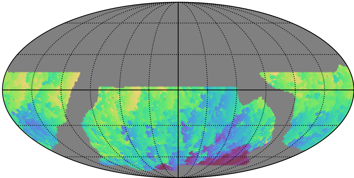
baseline_v2.1_10yrs WFD u band: Min HA
