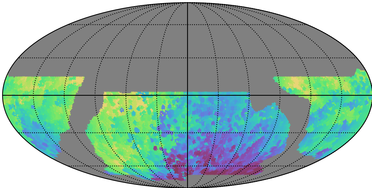
baseline_v2.1_10yrs WFD r band: Min HA
