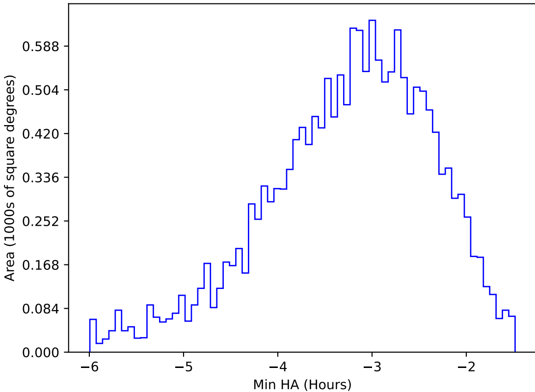
baseline_v2.1_10yrs WFD i band: Min HA
