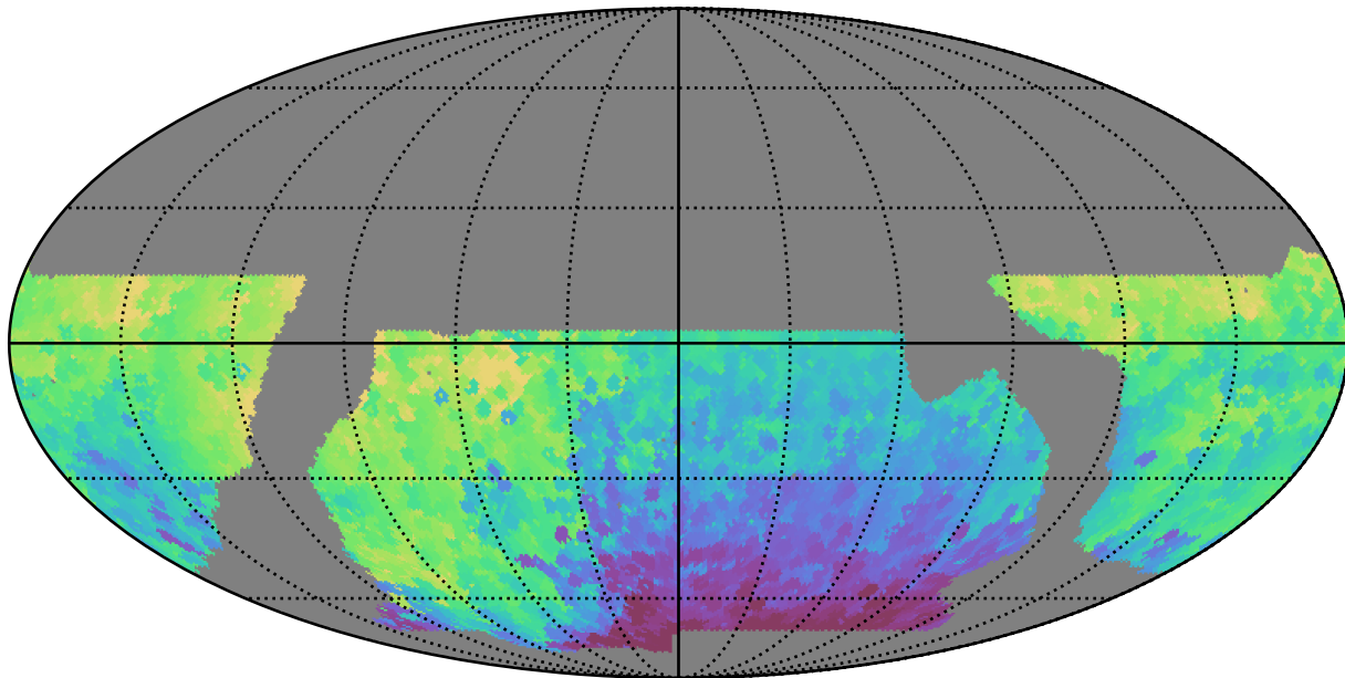
baseline_v2.1_10yrs WFD all bands: Min HA
