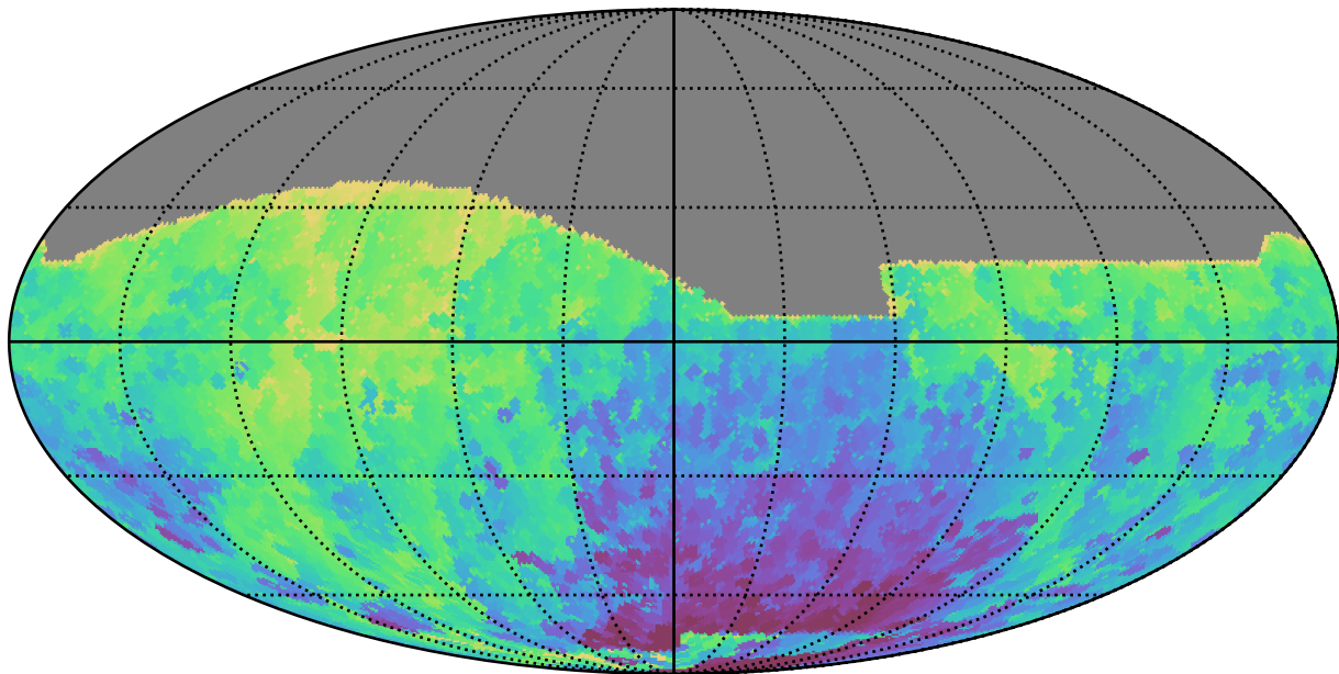
baseline_v2.1_10yrs All sky z band: Min HA
