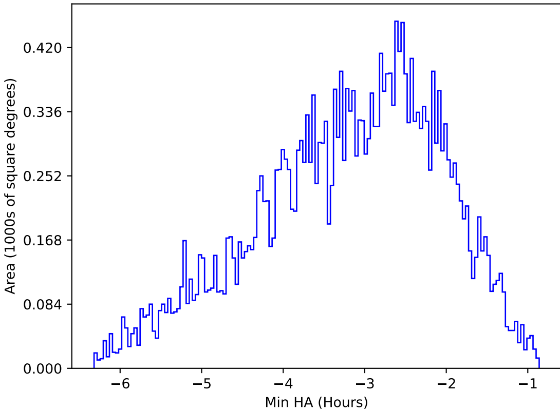
baseline_v2.1_10yrs All sky z band: Min HA
