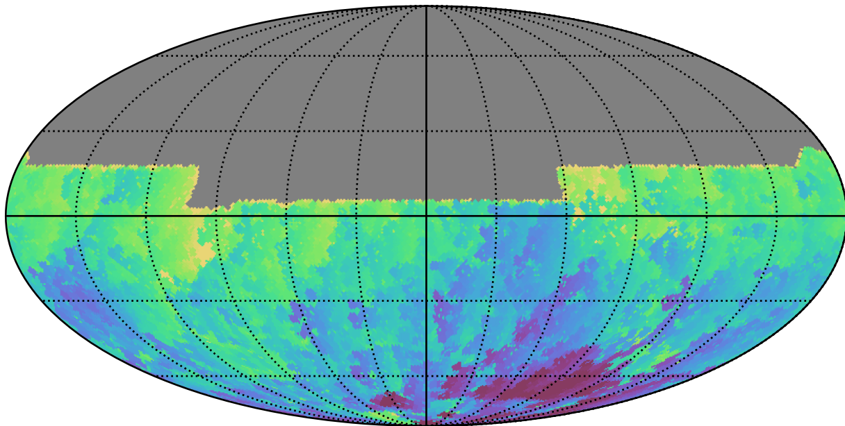
baseline_v2.1_10yrs All sky u band: Min HA
