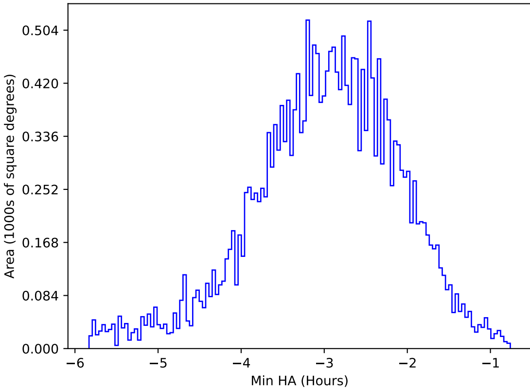
baseline_v2.1_10yrs All sky u band: Min HA
