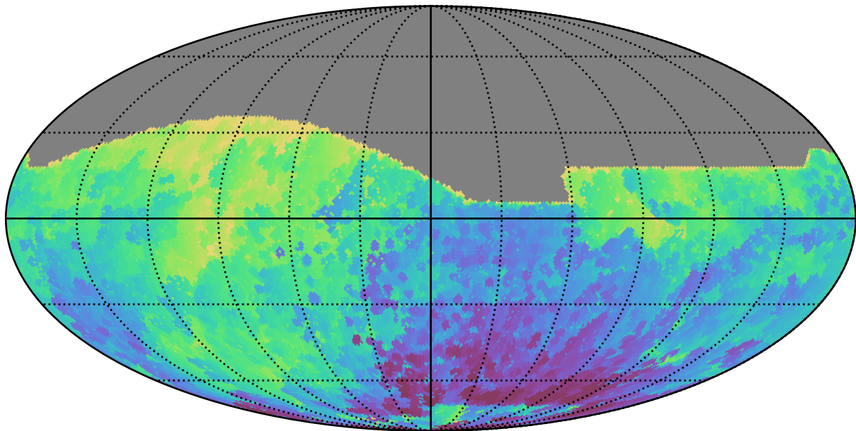
baseline_v2.1_10yrs All sky r band: Min HA
