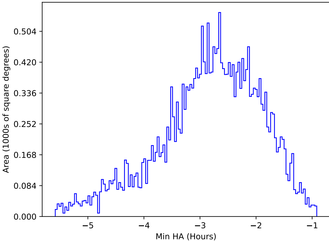
baseline_v2.1_10yrs All sky g band: Min HA
