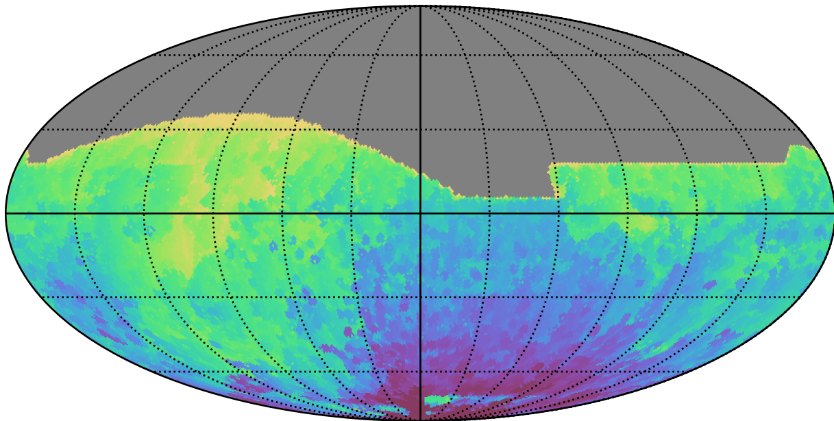
baseline_v2.1_10yrs All sky all bands: Min HA
