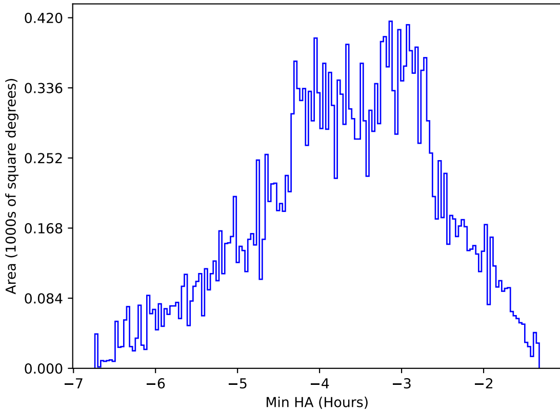
baseline_v2.1_10yrs All sky all bands: Min HA
