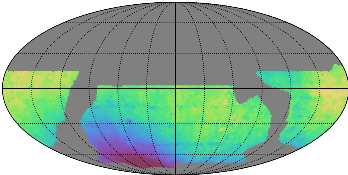
baseline_v2.1_10yrs WFD z band: Median solarElong
