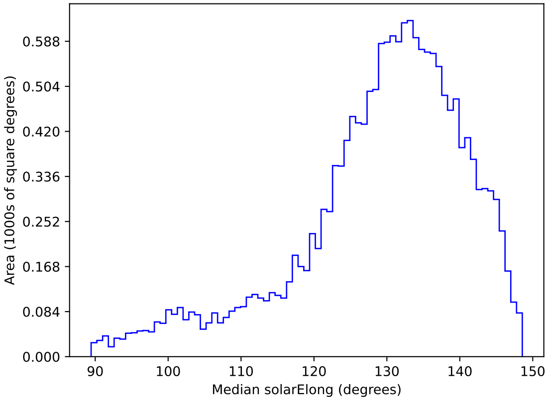
baseline_v2.1_10yrs WFD z band: Median solarElong
