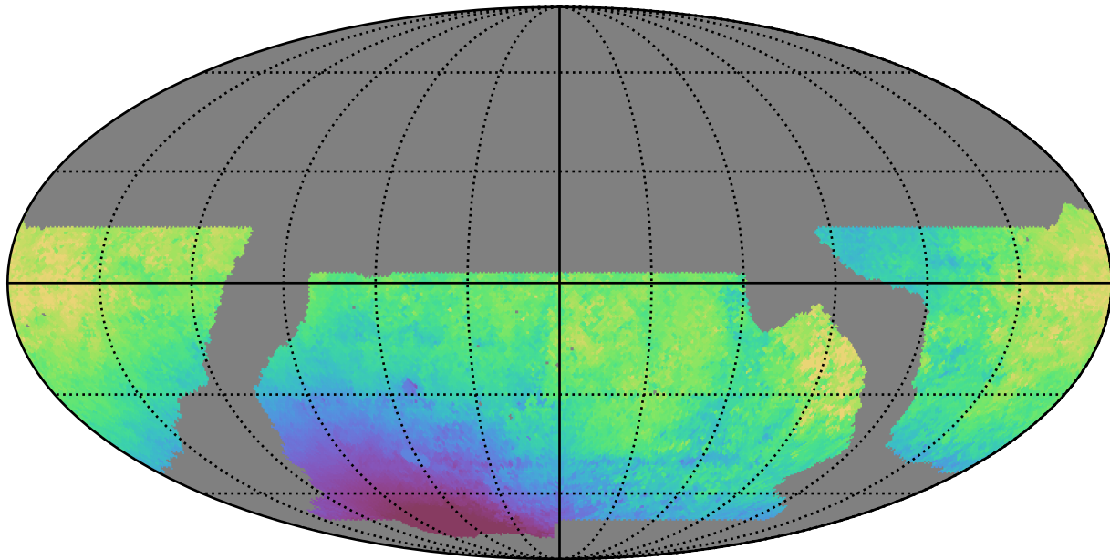
baseline_v2.1_10yrs WFD y band: Median solarElong
