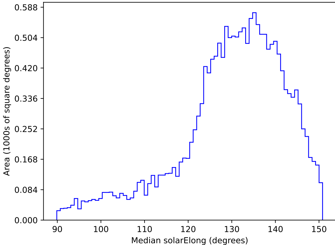
baseline_v2.1_10yrs WFD y band: Median solarElong
