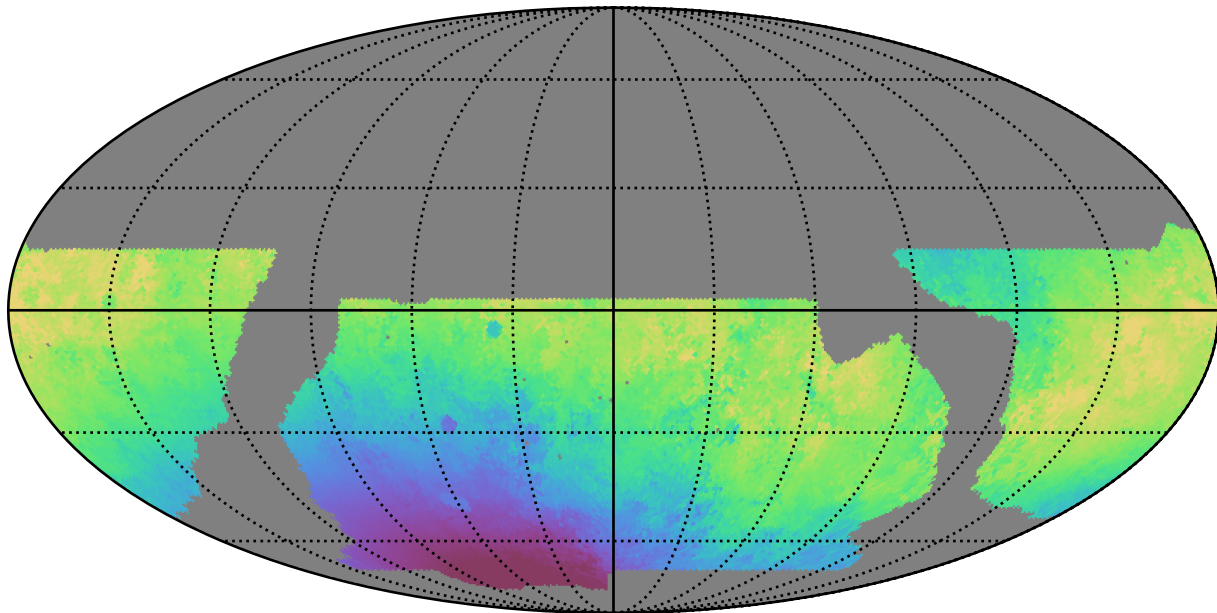
baseline_v2.1_10yrs WFD u band: Median solarElong
