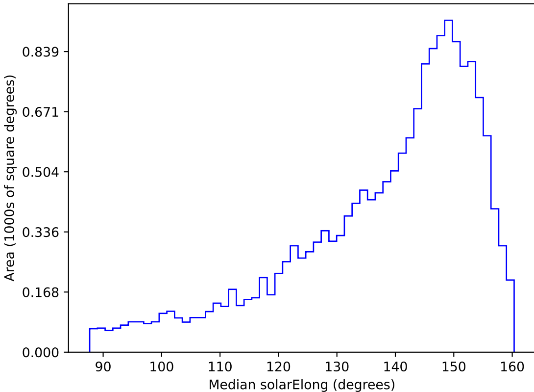
baseline_v2.1_10yrs WFD u band: Median solarElong
