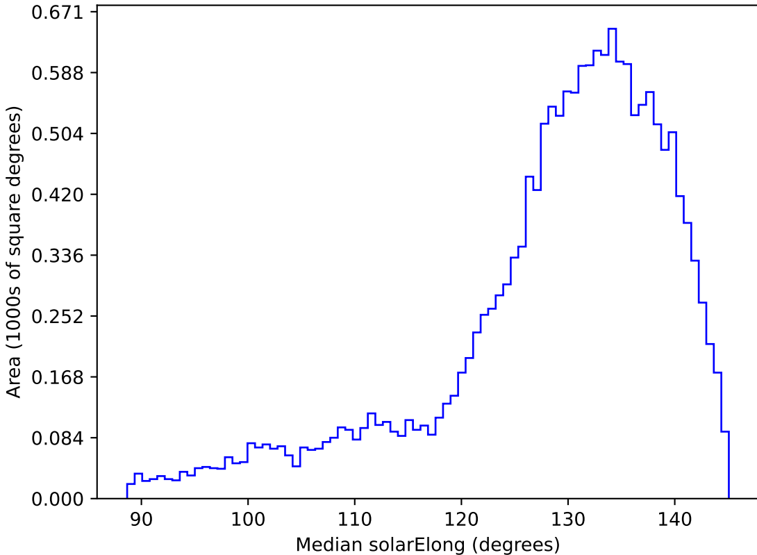
baseline_v2.1_10yrs WFD i band: Median solarElong
