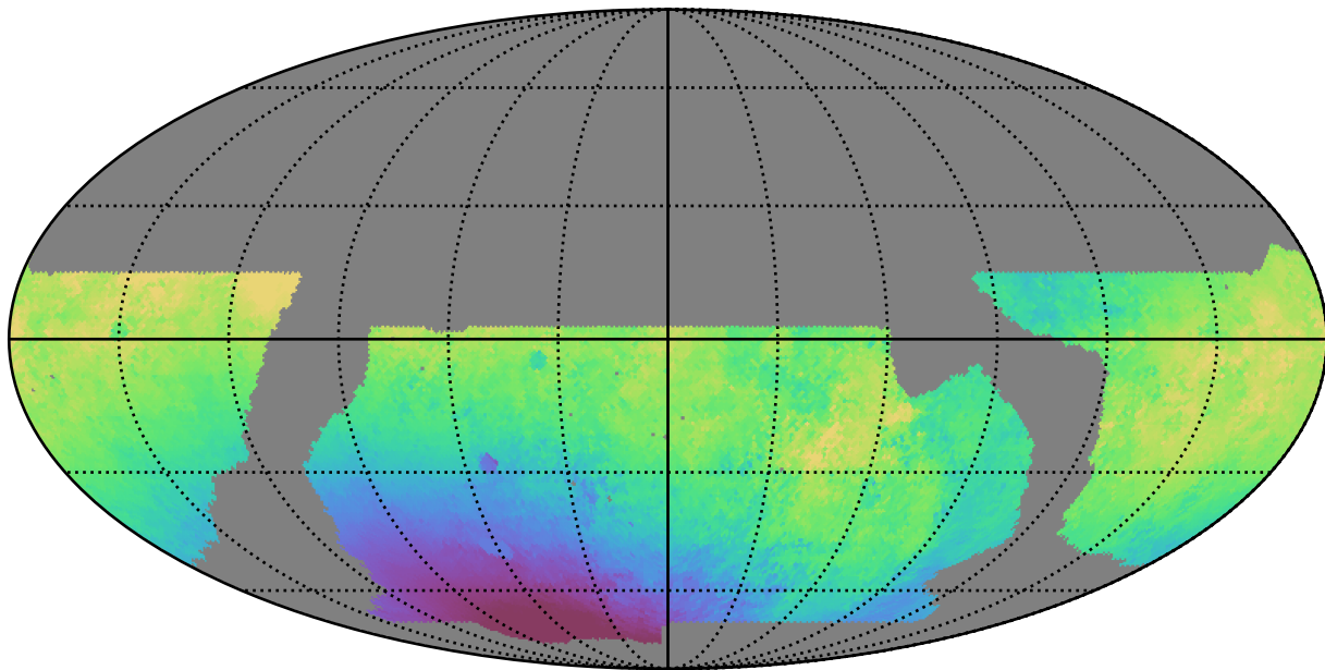
baseline_v2.1_10yrs WFD g band: Median solarElong
