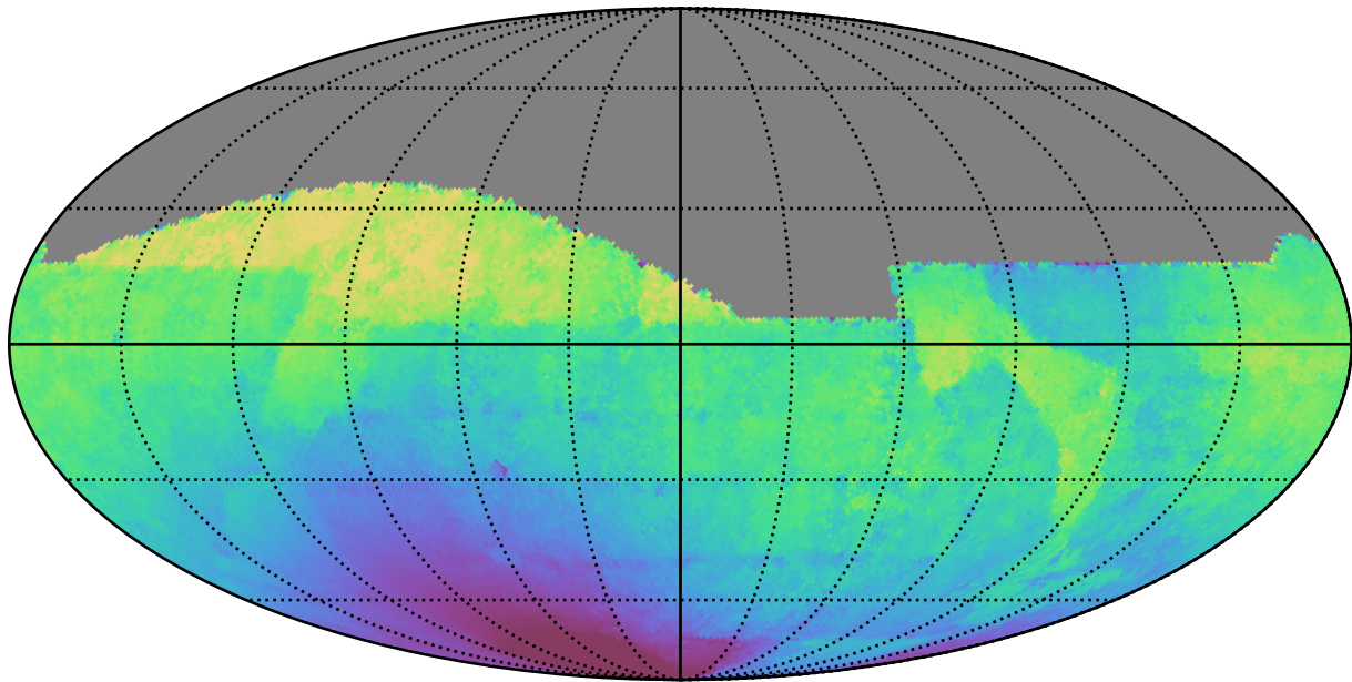
baseline_v2.1_10yrs All sky z band: Median solarElong
