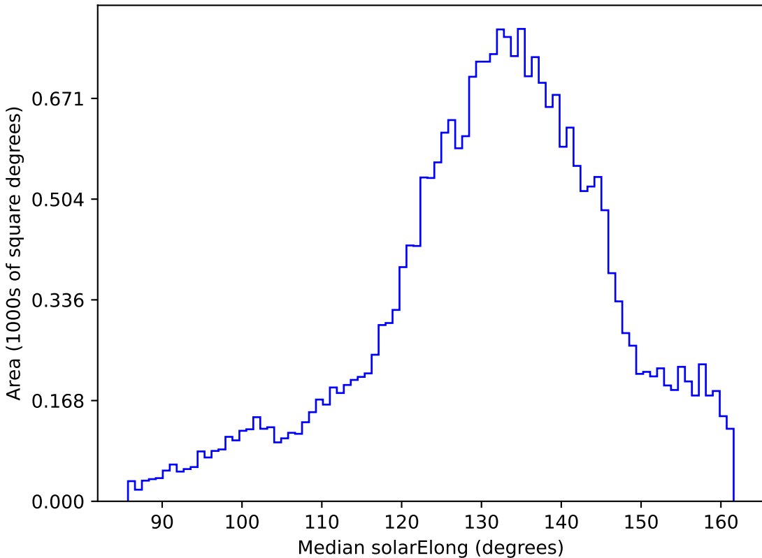
baseline_v2.1_10yrs All sky z band: Median solarElong
