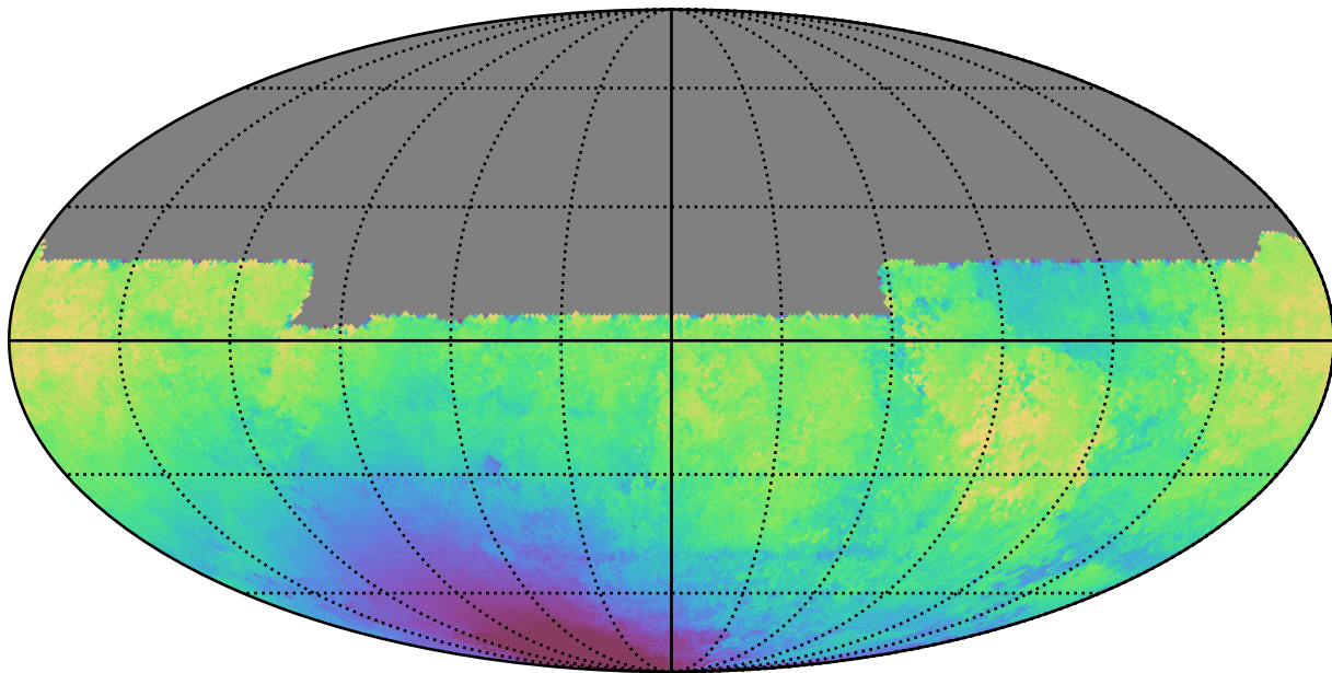
baseline_v2.1_10yrs All sky y band: Median solarElong
