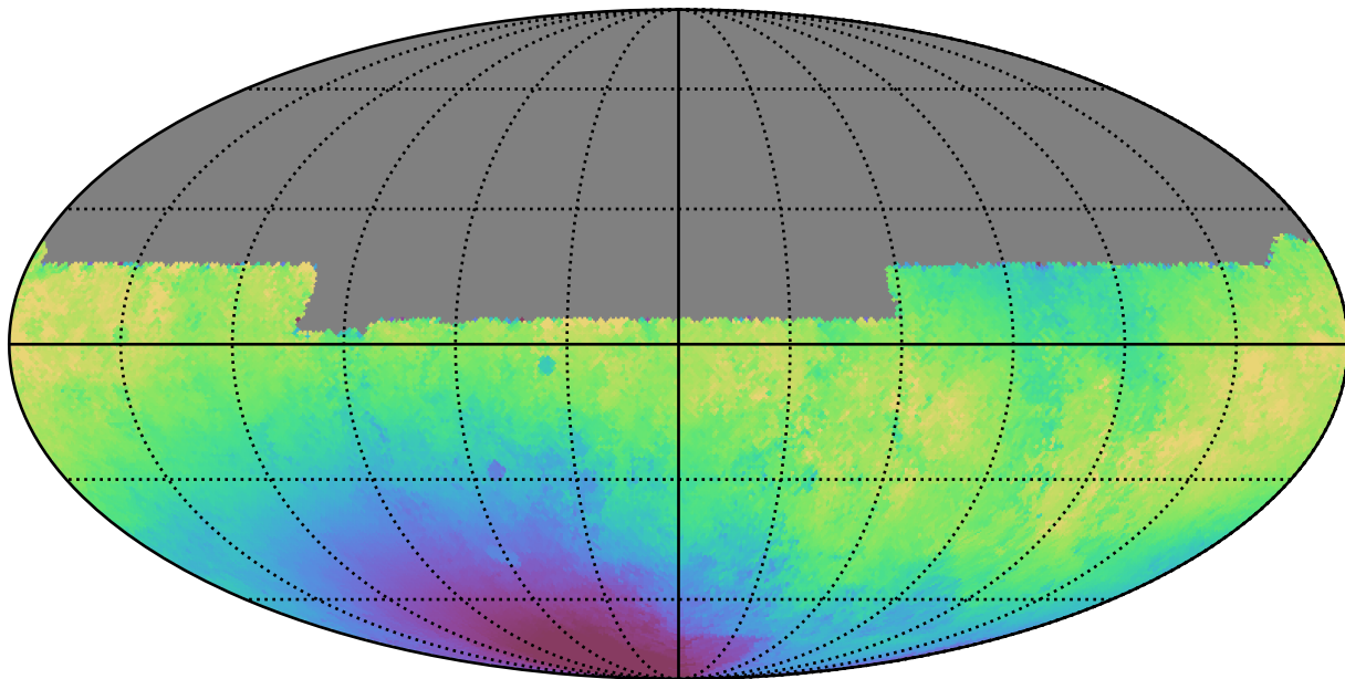
baseline_v2.1_10yrs All sky u band: Median solarElong
