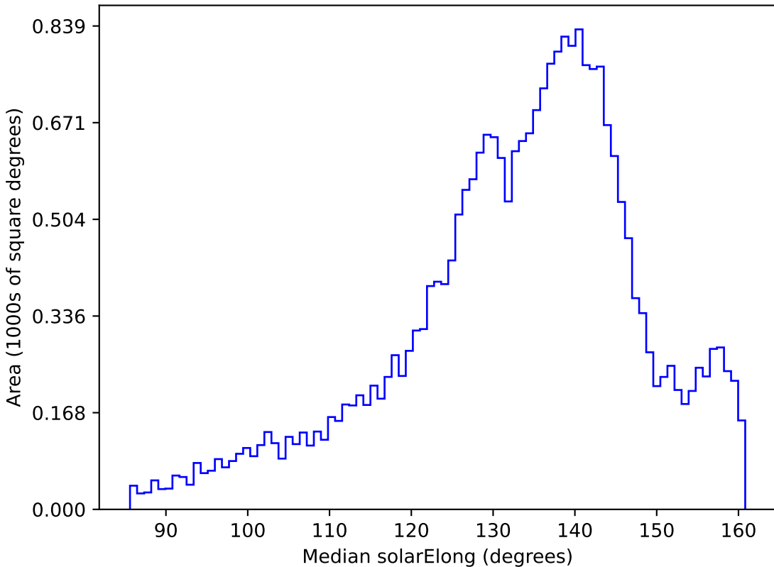
baseline_v2.1_10yrs All sky r band: Median solarElong
