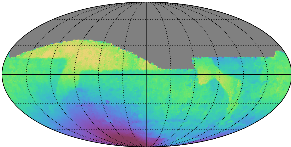
baseline_v2.1_10yrs All sky i band: Median solarElong
