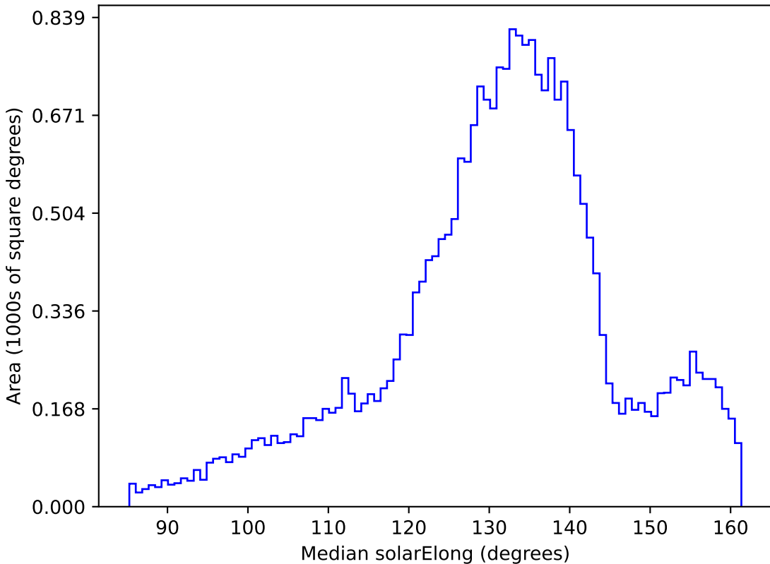
baseline_v2.1_10yrs All sky i band: Median solarElong
