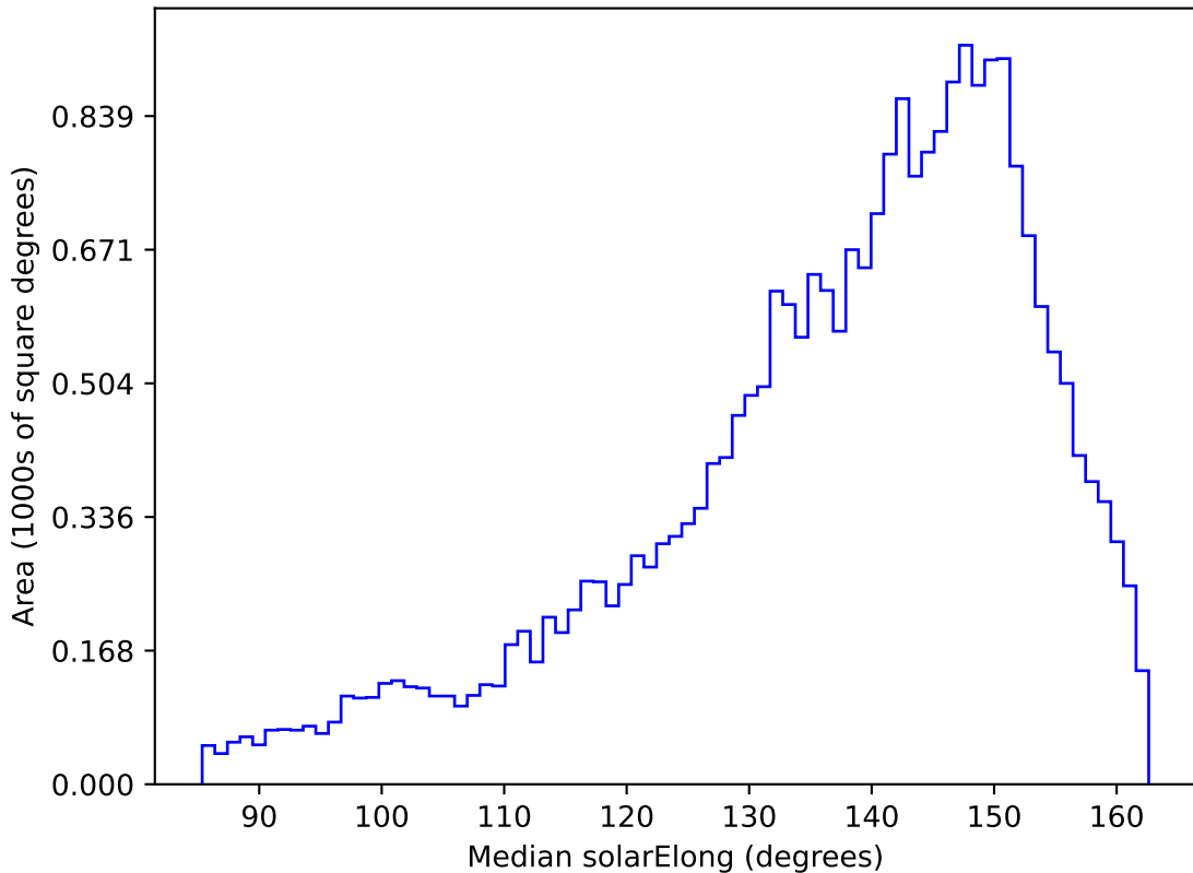
baseline_v2.1_10yrs All sky g band: Median solarElong
